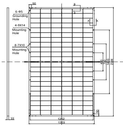
Rear View
